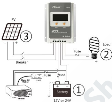
Figure 2-1 Montage
