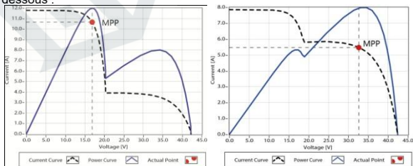
Figure 1-3 Courbe Mutil-MPP
